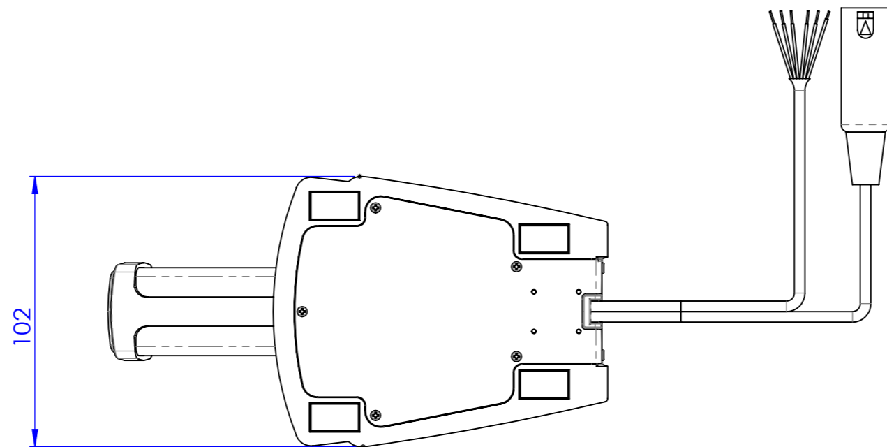
AT882TL/D3RC5 & DS3RC5 Outline drawing Scale 1 : 2
